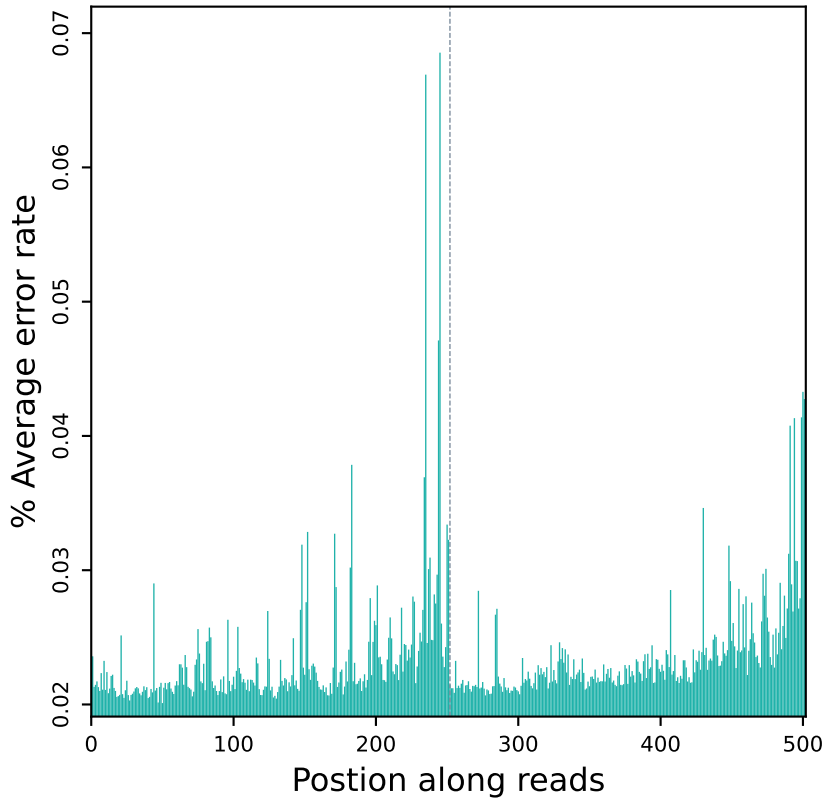
Error rate distribution along reads (R10714)
